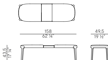
942/01 panca \ bench
