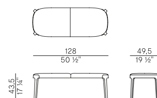
942/02 panca \ bench
